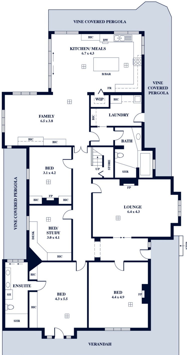
GROUND FLOOR
